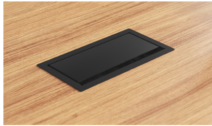
Rectangular conduit. Metallic hatch access to the lower part of the table for wooden table tops. Metal frame available in black or grey and central part in the veneer of the finish of the table. Does not include power options. Dimensions: 32x15 cm | 12.59"x5.90"
